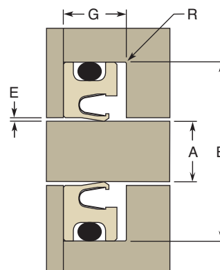
Rotary Seal
