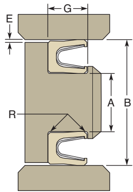
Piston Seal
