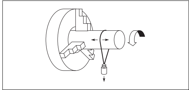
Figure 2-26. String Test for Shaft Lead
