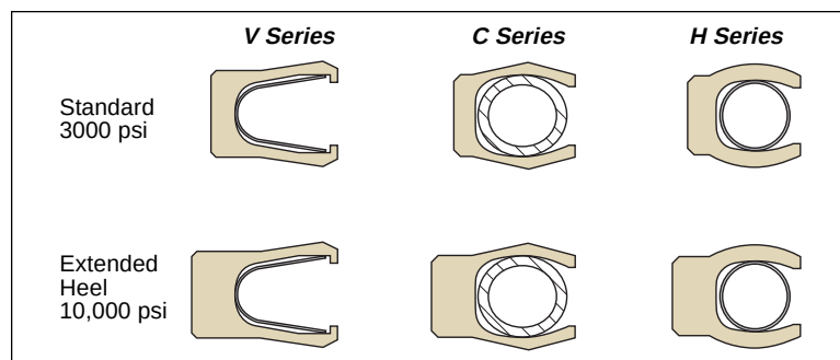
Figure 2-12. High Pressure Seals
