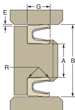
Piston Seal
