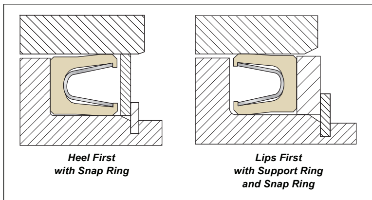
Figure 2-5. Alternative Installations
