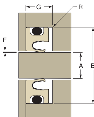
Rotary Seal
