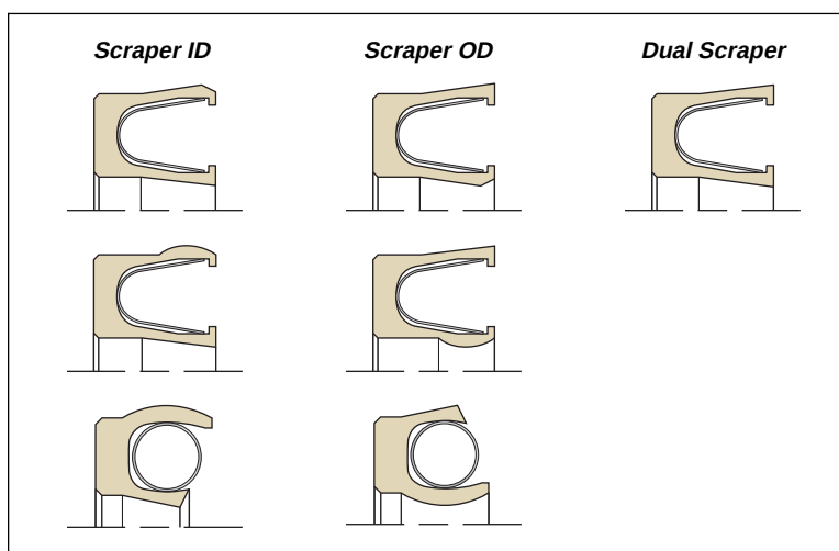
Figure 2-20. Scraper Lips
