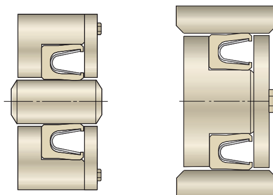
Two-Piece Rod and Piston Glands
