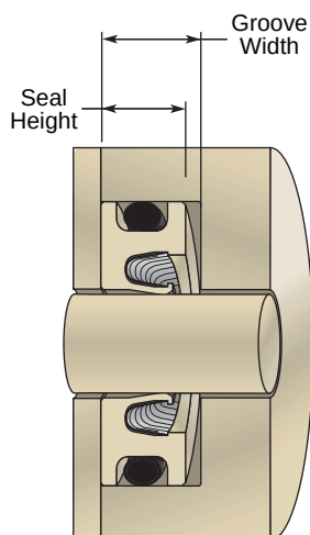
Rotary Application
